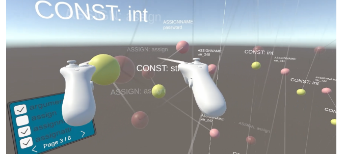
Figure 14. AST nexus filtering (assign nodes are ghosted since deselected).
