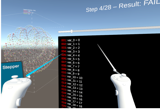
Figure 11. Replay synchronized AST nexus (left) shows reduced input set for Step 4 of 28 on screen (red line numbers indicate set in testcase failure).
