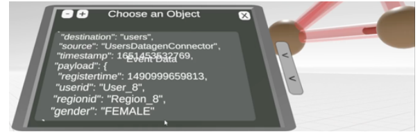
Figure 9. Example event details after selecting red capsule.
