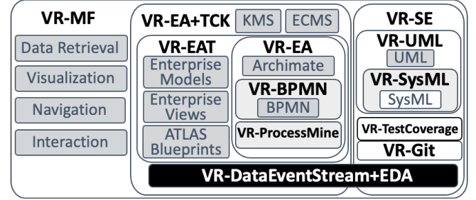
Figure 1. The VR-EDStream+EDA solution concept (black) in relation to our prior VR solution concepts.
