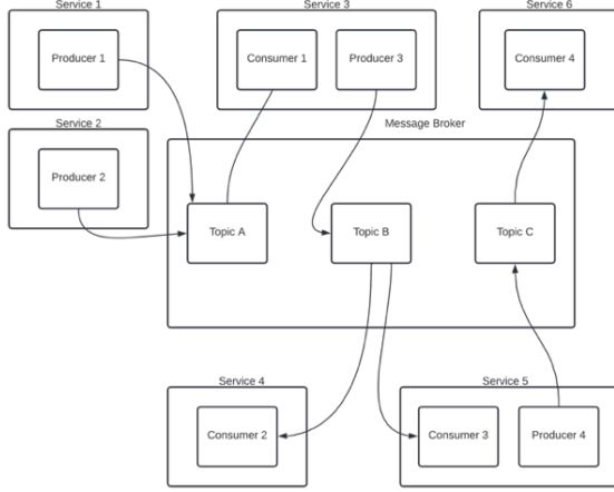
Figure 2. Example EDA couplings between services.
