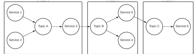
Figure 10. Abstracted node grouping EDA example.
