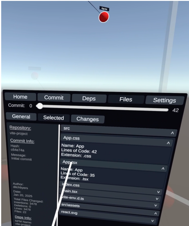
Figure 20. VR-Tablet: Git Files Tab: Files contained in selected src folder.
