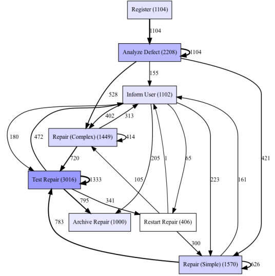
Figure 4. Example DFG-based process map result from pm4py.
